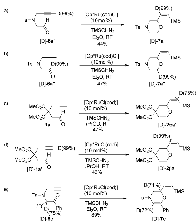
Scheme 2. Deuterium-labeling experiments.
